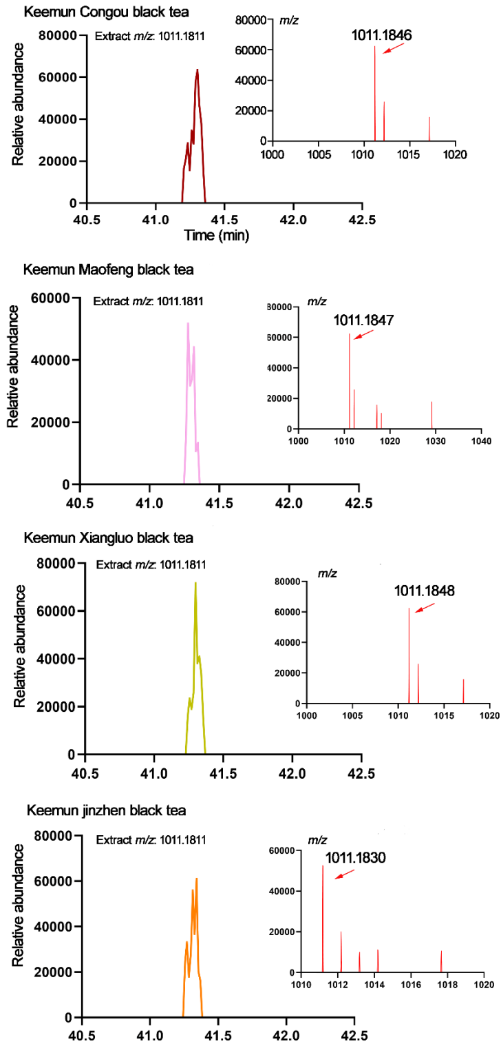
Figure S1. The 1011.1811 m/z ion chromatogram extracted from MS data of the four Keemun black tea infusions.
