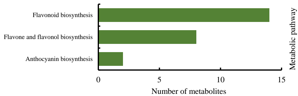
Fig. S3 The differential metabolites of flavonoids were enriched by KEGG pathway ( P < 0.05 ). Flavonoid biosynthesis is the pathway of ko00941. Flavone and flavonol biosynthesis is the pathway of ko00944. Anthocyanin biosynthesis is the pathway of ko00942.
