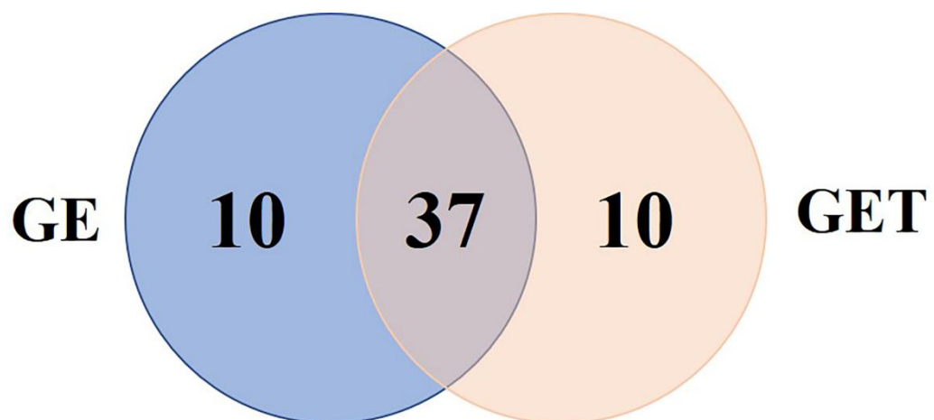
Figure S4. The Venn diagram of volatile components in GE and GET with OAV > 1.
