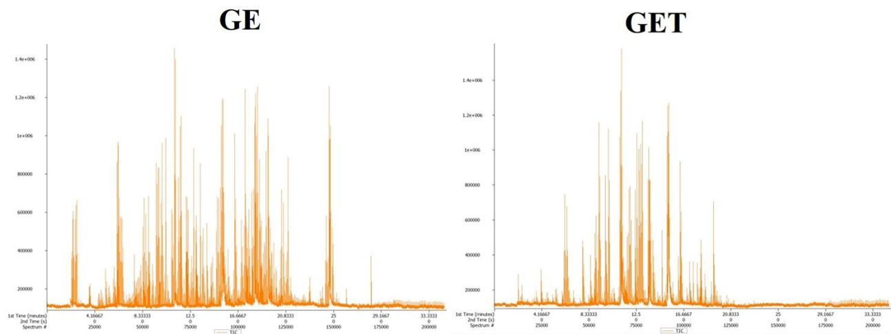
Figure S3. The total ion chromatograms of GE and GET obtained from GC × GC-TOFMS.
