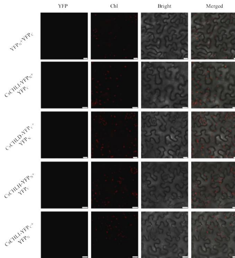
Fig. S1 BiFC of free YFP C or YFP N coexpressed with CsCHLI, CsCHLD, and CsCHLH. YFP Fluorescence (YFP), chlorophyll autofluorescence (Chl), bright-field (Bright), and Merged images (Merged). The scale bar is 20 μm.
