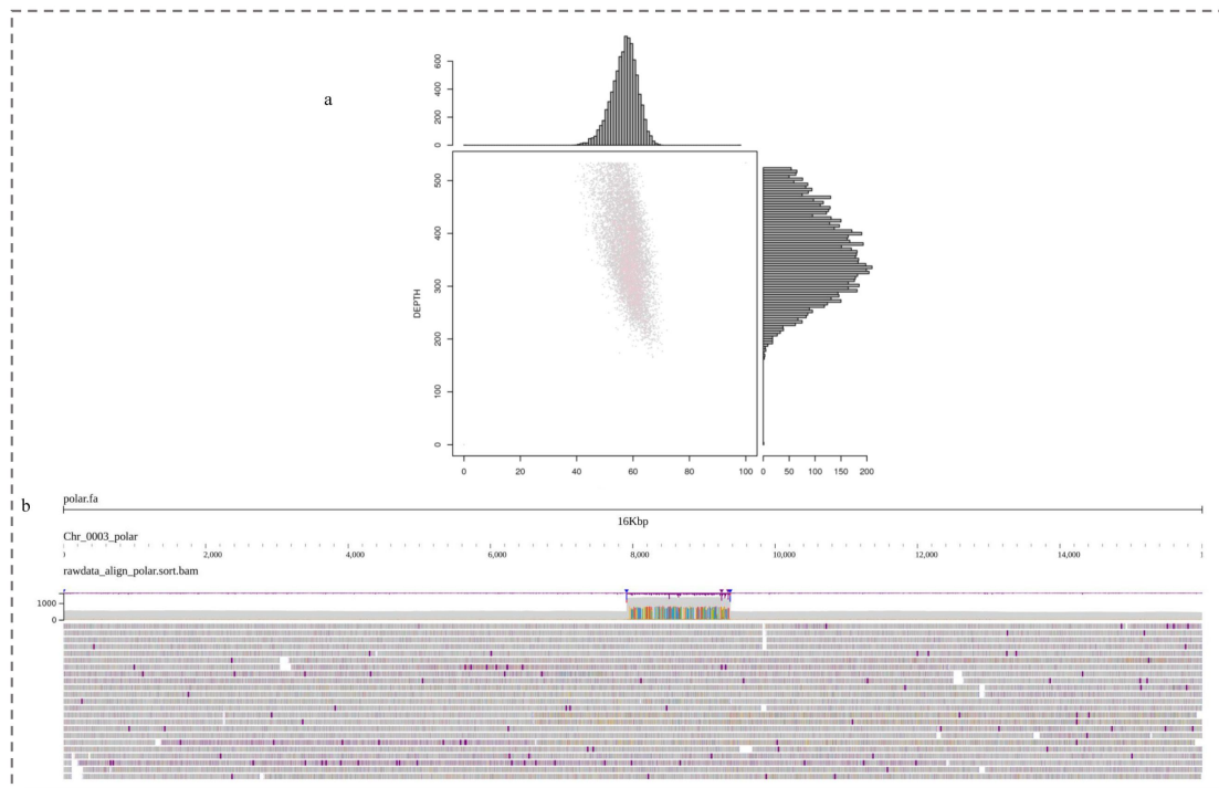
Fig S2. The GC depth map and reads comparison map showed the quality of the assembly. The horizontal axis showed the GC content and the vertical axis showed the sequencing depth, with the sequencing depth distribution on the right and the GC content distribution on the top in GC depth map (a), Most of the reads in the reads comparison map were well connected to the end and the first end (b).
