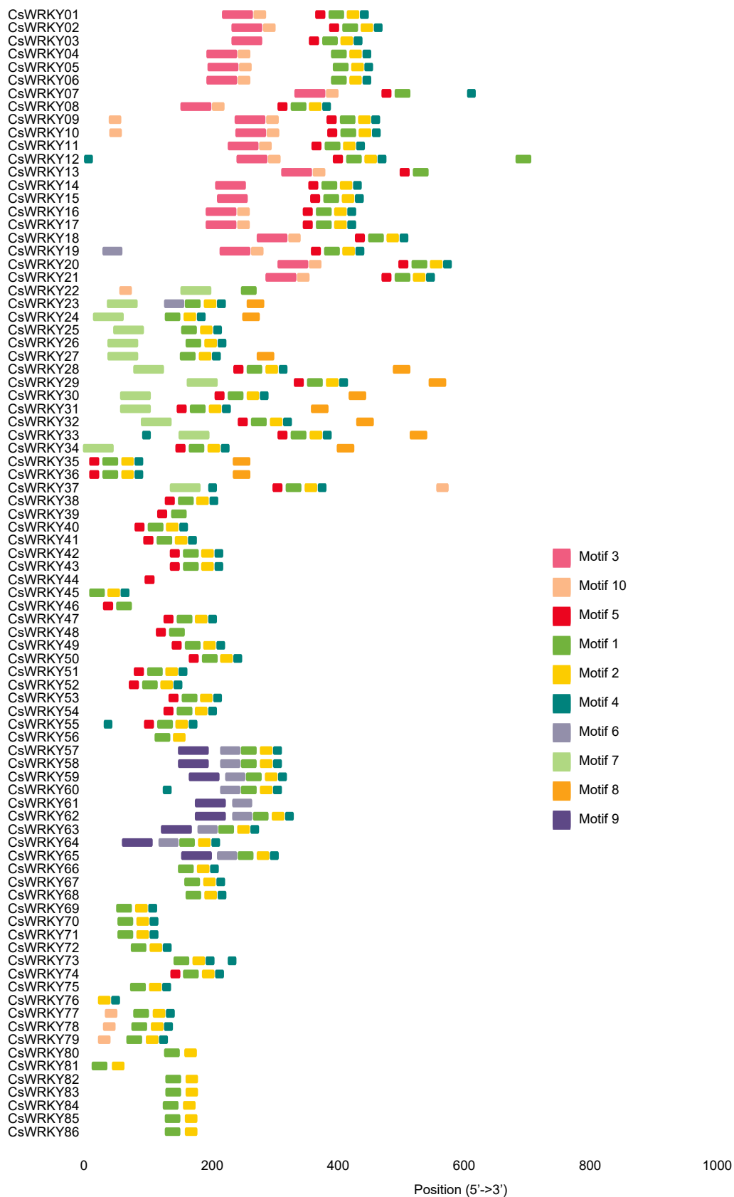
Supplemental Figure 1. Conserved motifs of the WRKY genes of tea plants. The conserved motifs were investigated by MEME. Top 10 of the motifs are shown.
