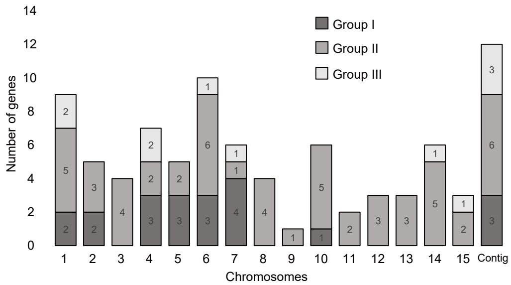
Supplemental Figure 5. Chromosome distributions of tea plant WRKY genes. The number of WRKY genes from each group are shown on the 15 chromosomes and unanchored contigs of tea plant genome. The x-axis indicates the chromosome, while the y-axis represents the number of WRKY genes.
