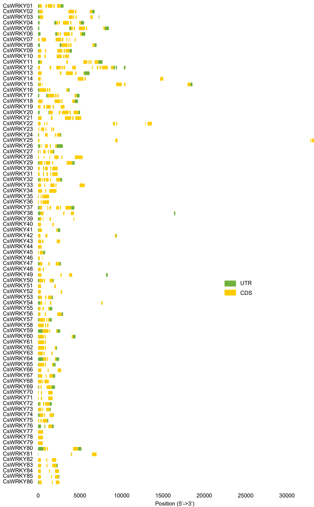
Supplemental Figure 2. Intron–exon structures of the tea plant WRKY genes. Yellow boxes, green boxes and lines represent exons, UTRs and introns, respectively.
