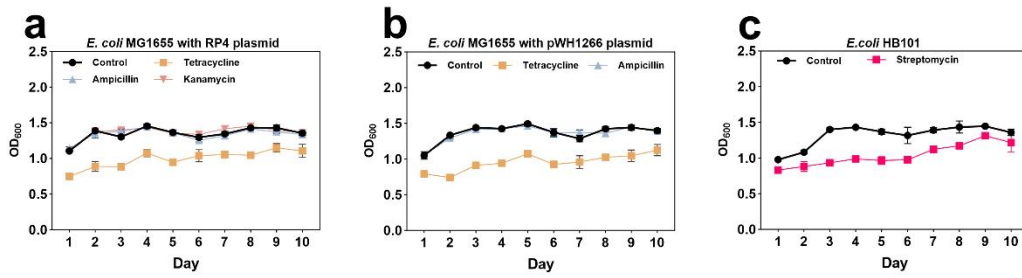
Supplementary Fig. S2. The growth curves of three bacterial strains under antibiotic pressure (CON: control group): (a) E. coli with RP4 plasmid. (b) E. coli with the pWH1266 plasmid. (c) E. coli HB101.
