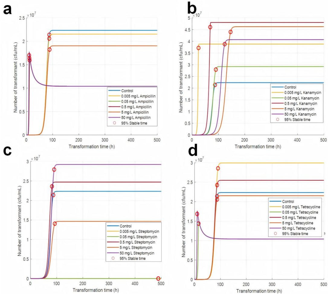
Supplementary Fig. S7. Trajectories of transformant prevalence under the exposure of antibiotics at environmentally relevant concentrations.
