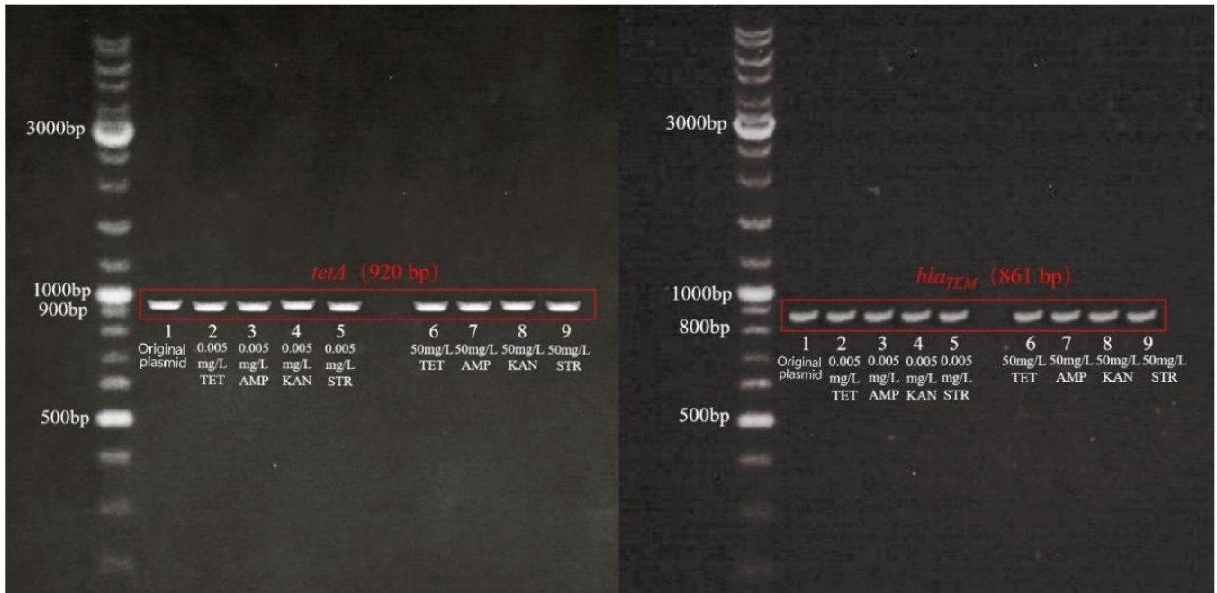
Supplementary Fig. S6. PCR electrophoresis images of the tetA and bla TEM genes in the transformants carrying the pWH1266 plasmid.
