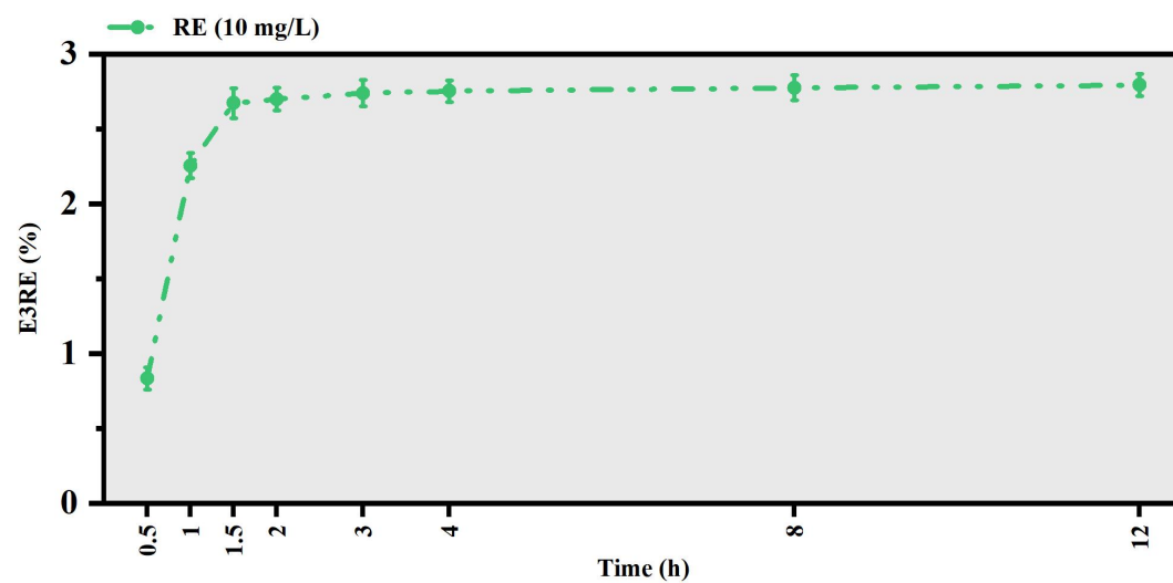
Fig. S5 Batch removal efficiencies (RE) of extracellular polymeric substances (EPS) adsorption for 10 mg/L E3.
