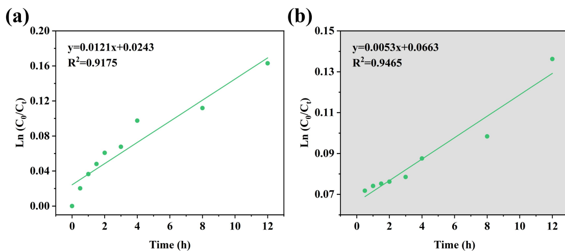
Fig. S4 First-order kinetics of E3 removal over a 12 h period. (a) Daytime and (b) nighttime fitting curves.
