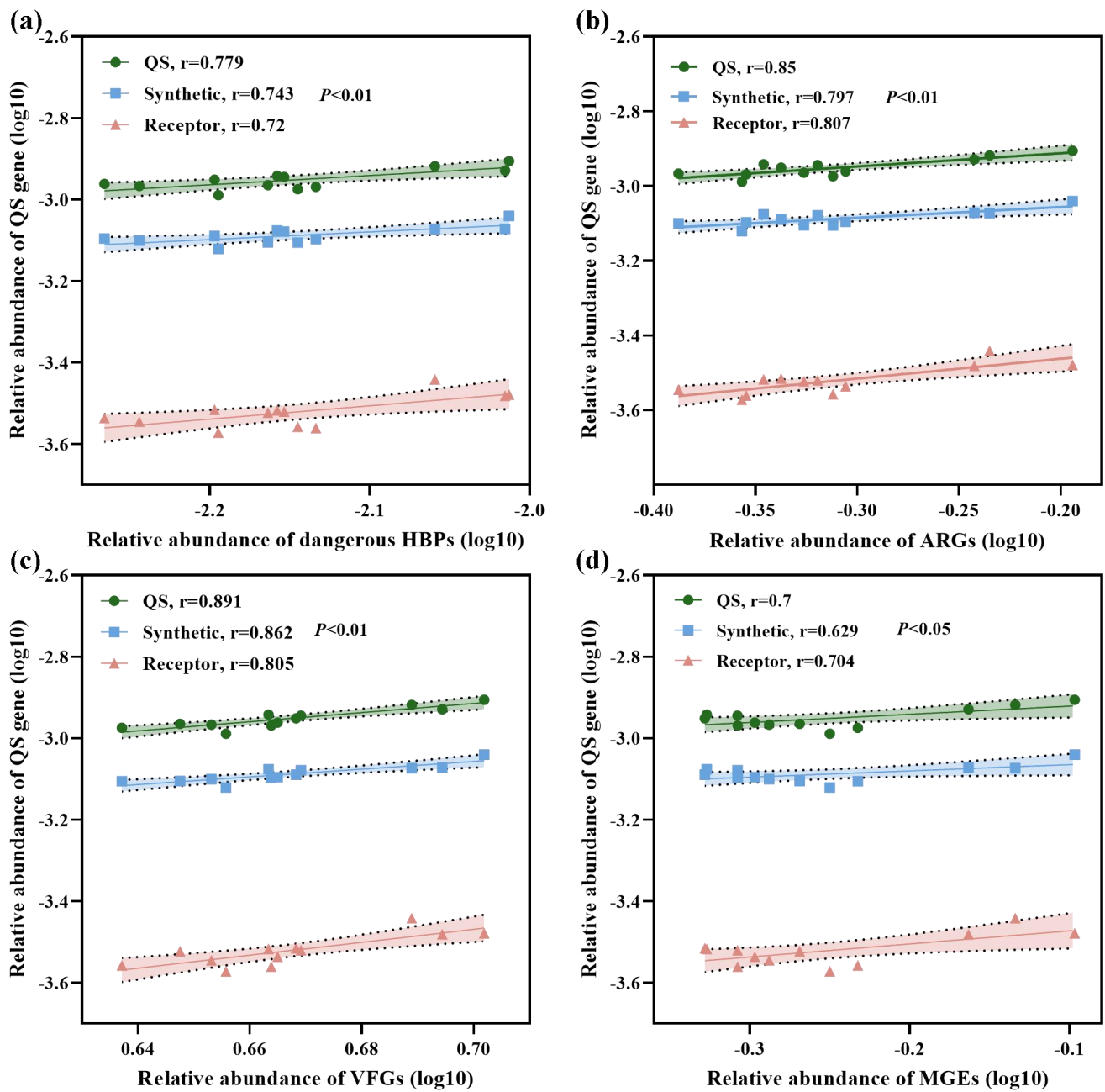
Supplementary Fig. S8. Linear regression analysis of QS-related gene abundance with (a) HBPs, (b) ARGs, (c) VFGs, and (d) MGEs.
