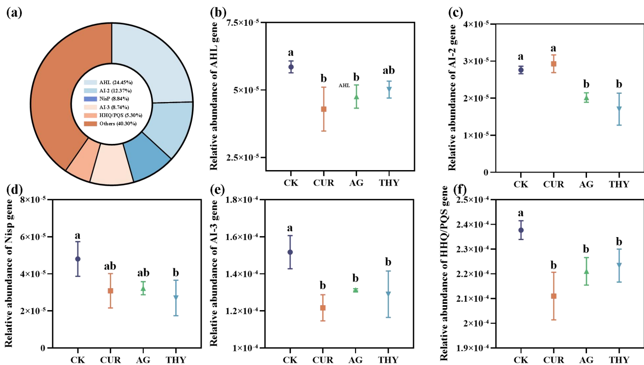
Supplementary Fig. S6. (a) The main QS gene categories in the soil. Effects of applying root exudates on the abundance of (b) AHL-class, (c) AI-2 class, (d) NISP-class, (e) AI-3 class, and (f) HHQ/PQS class genes. Different lowercase letters indicate significant differences among the treatments at p < 0.05 .
