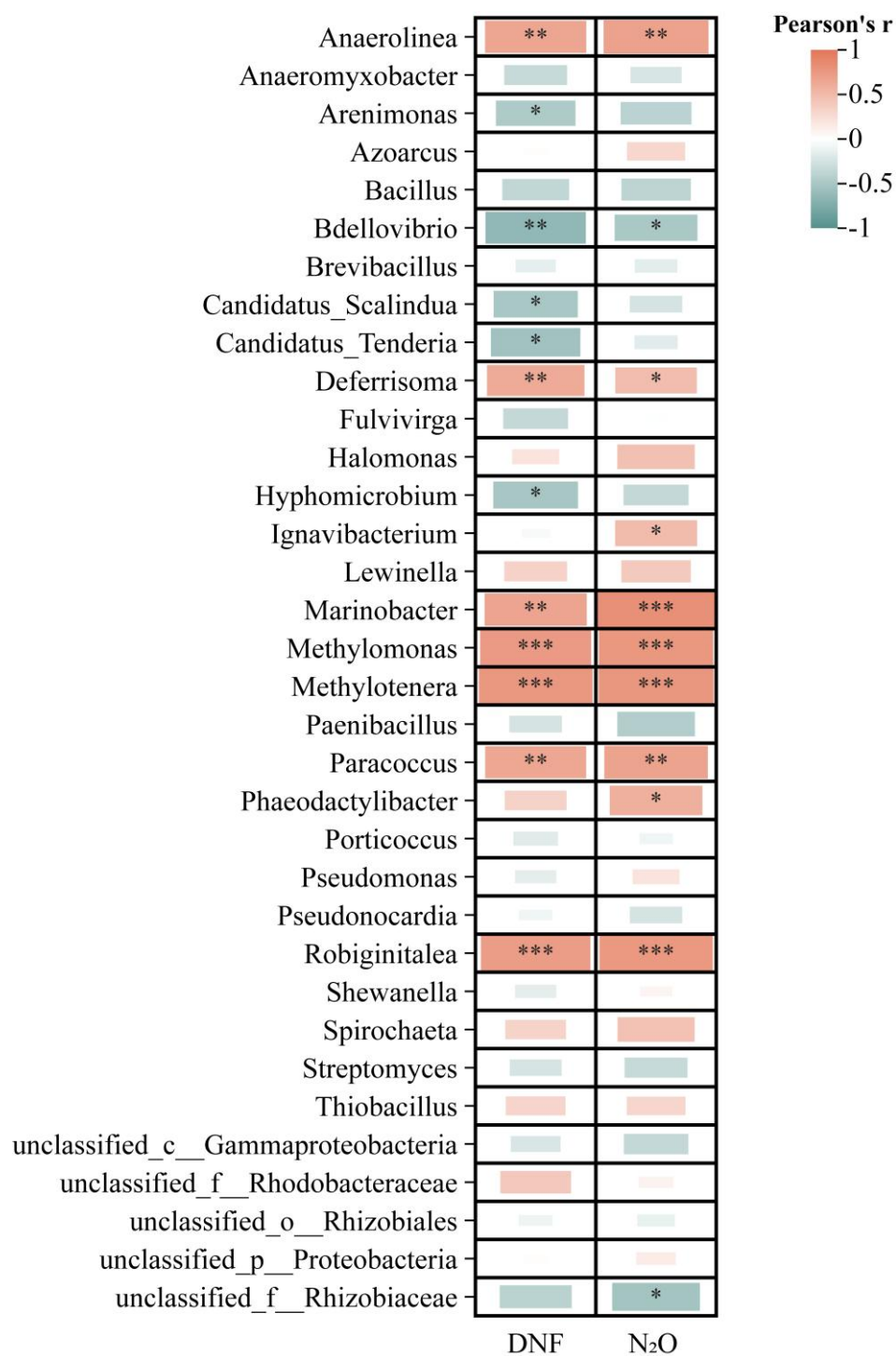
Fig. S3. Relationships between denitrifiers and the denitrification rates and N 2 O emission rates after incubation. DNF is the potential denitrification rate. * represents p < 0.05 ; ** represents p < 0.01 ; *** represents p < 0.001 .
