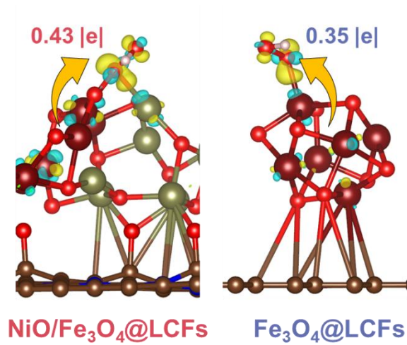
Supplementary Fig. S9 The differential charge density plot of OOH adsorbed on Fe 3 O 4 @LCFs and NiO/Fe 3 O 4 @LCFs.
