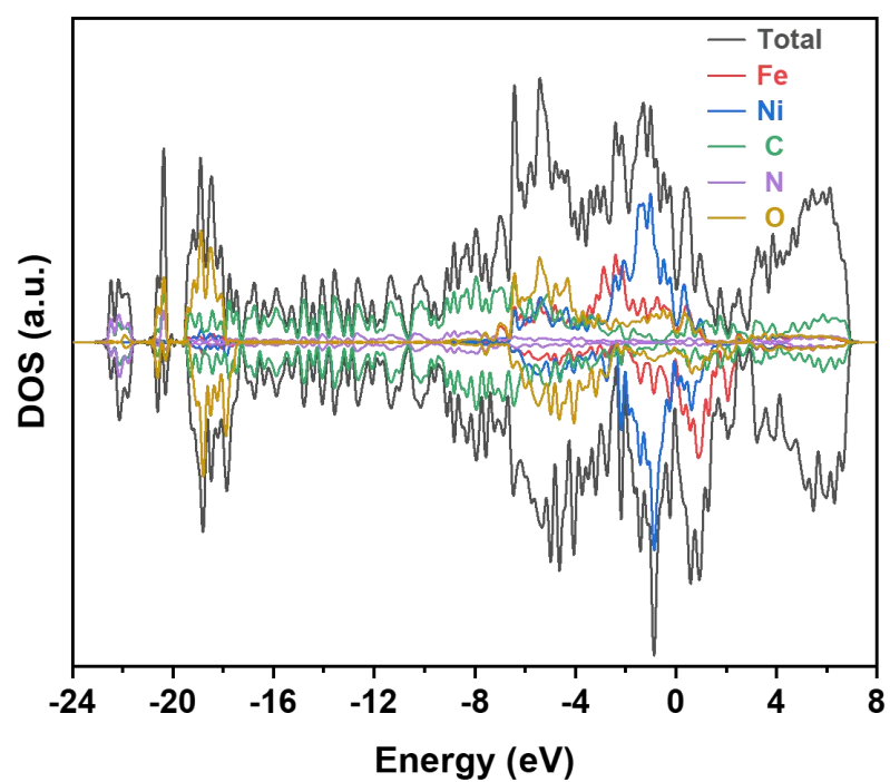
Supplementary Fig. S8 Density of states of NiO/Fe 3 O 4 @LCFs.
