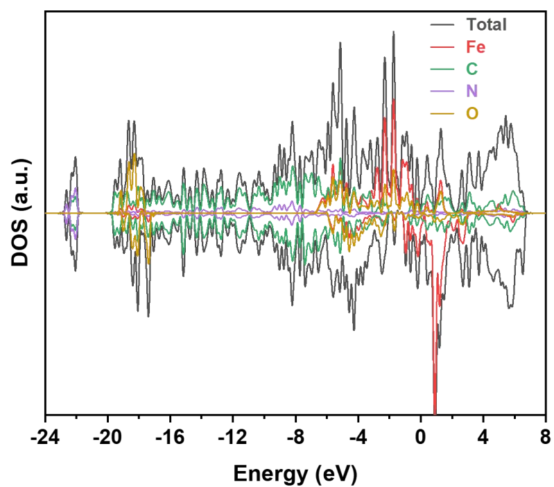
Supplementary Fig. S7 Density of states of Fe 3 O 4 @LCFs.
