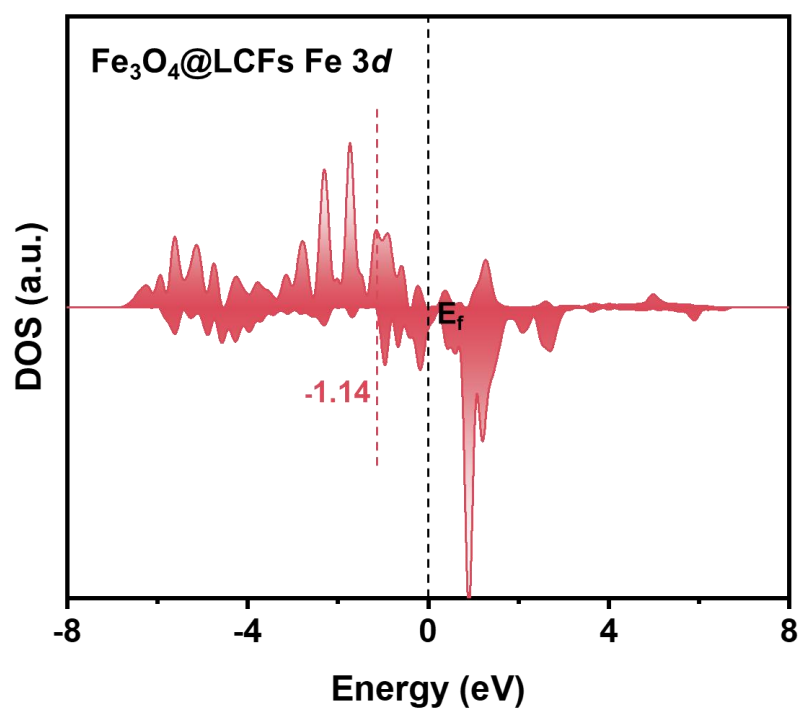
Supplementary Fig. S6 Density of states onto Fe 3d orbitals for Fe 3 O 4 @LCFs.
