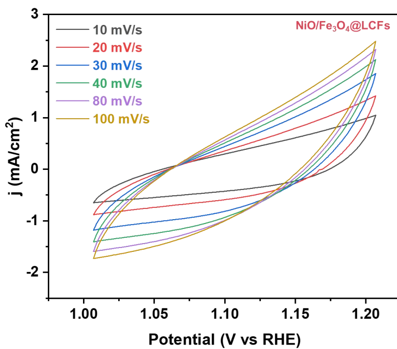
Supplementary Fig. S3 The ECSA of \text{NiO/Fe}_3\text{O}_4@\text{LCFs} .
