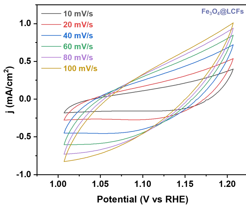
Supplementary Fig. S2 The ECSA of \text{Fe}_3\text{O}_4@\text{LCFs} .
