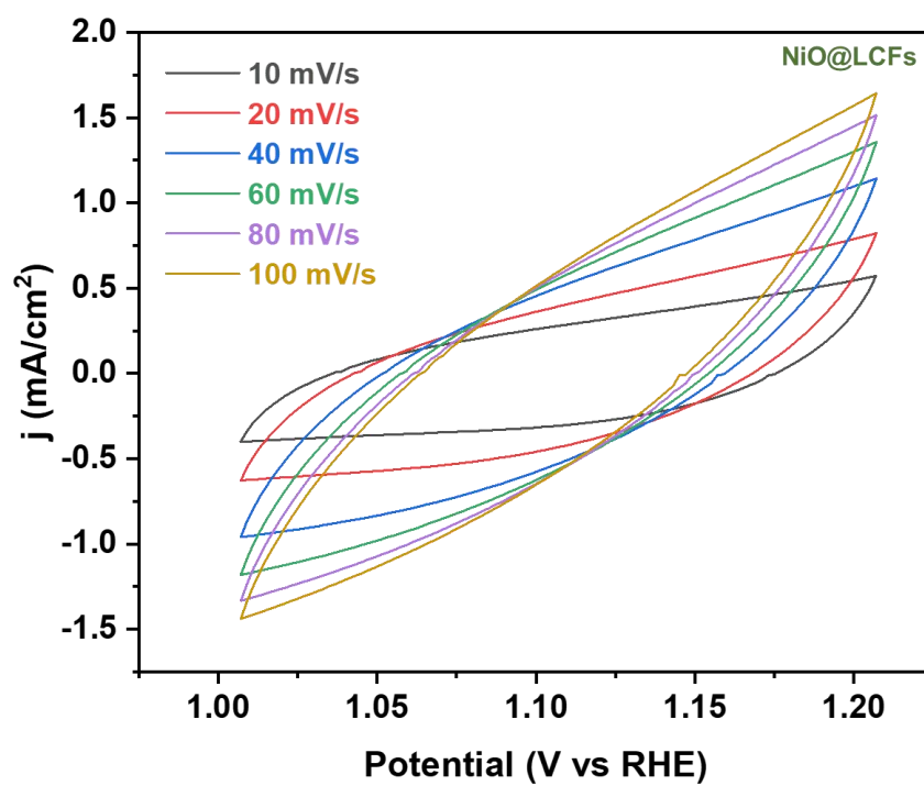
Supplementary Fig. S1 The ECSA of NiO@LCFs.
