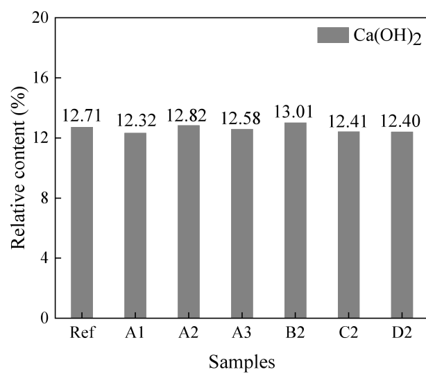
Fig. S1 Semi-quantitative XRD analysis of \text{Ca(OH)}_2 .
