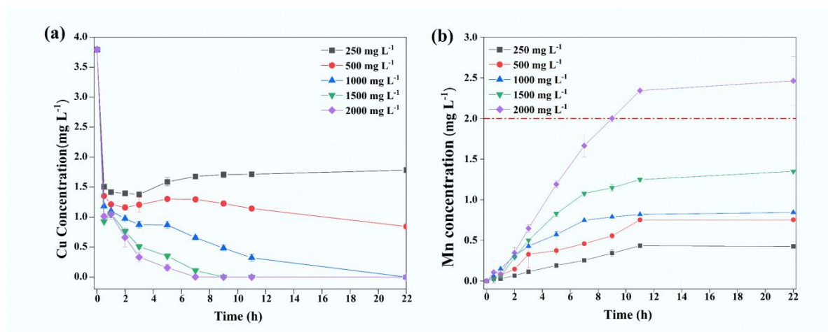
Fig. S2 The Cu concentration (a) and Mn dissolution concentration (b) varied with time under different dosage of modified biochar.
