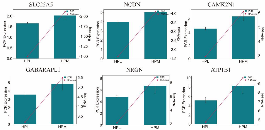
Figure S2. qPCR validation of the GABA-related genes. These findings support the reproducibility and reliability of the transcriptome data.
