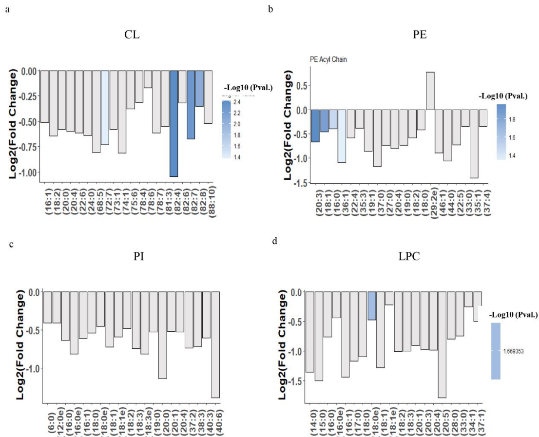
Figure S2. The acyl chain saturation levels of glycerophospholipids in the longissimus thoracis . a) The intensity fold changes of individual fatty acyl chains associated with CLs sorted by the degree of saturation. b) The intensity fold changes of individual fatty acyl chains associated with PEs sorted by the degree of saturation. c) The intensity fold changes of individual fatty acyl chains associated with PIs sorted by the degree of saturation. d) The intensity fold changes of individual fatty acyl chains associated with LPCs sorted by the degree of saturation.
