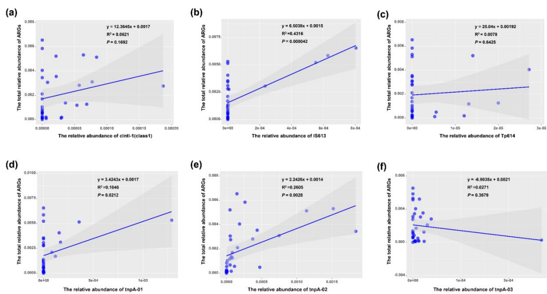
Fig. S1. Regression analysis of the relative abundance of MGEs and ARGs.
