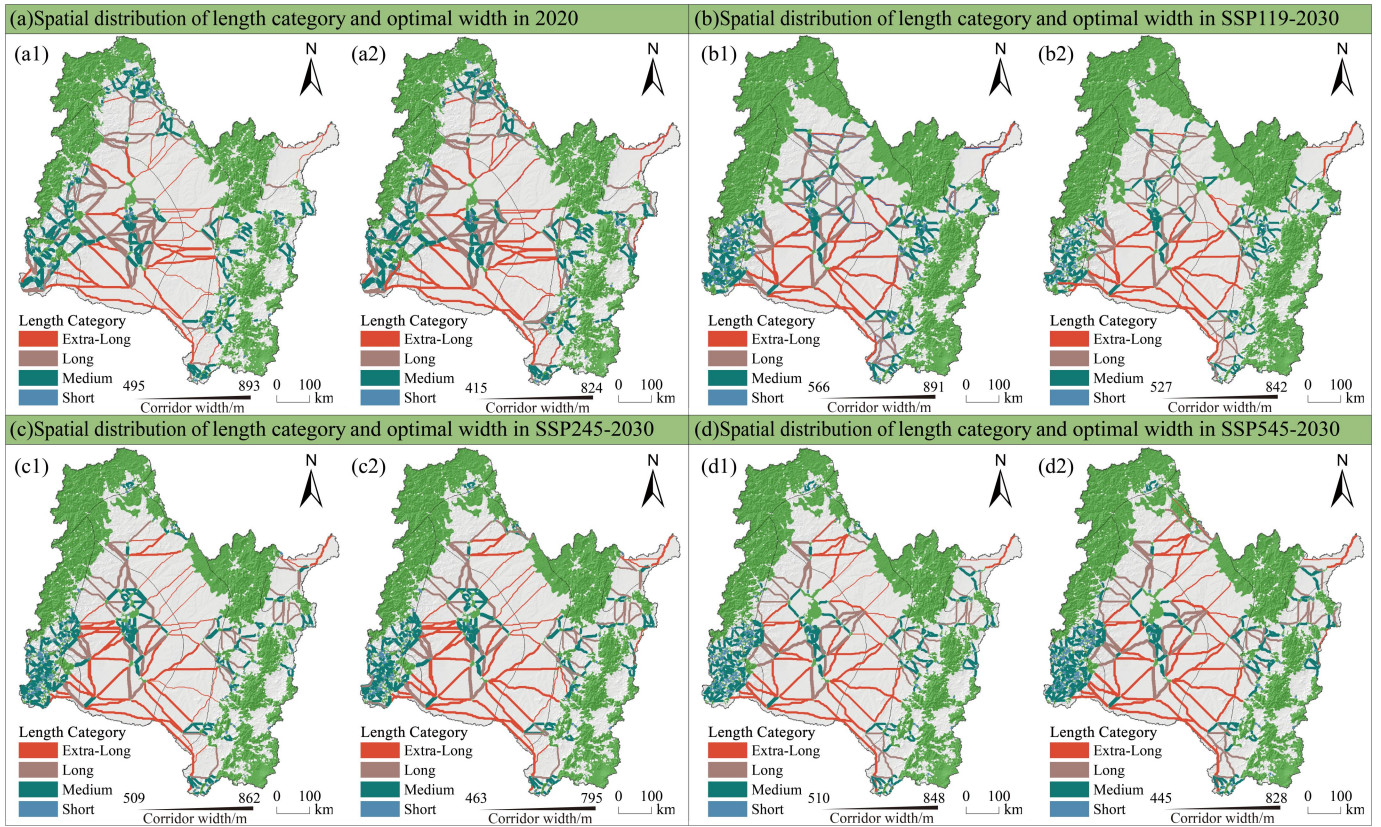
Supplementary Fig. S6 Spatial distribution of length category and optimal width in the SRB. For the figure panels, (a)–(d) represent the years 2020, SSP119-2030, SSP245-2030, SSP545-2030, respectively. Each panel is subdivided into two subpanels: the left subpanel presents existing ecological corridors classified by length categories (short, medium, long, and extra-long), while the right subpanel illustrates the optimized ecological corridors following the introduction of potential corridors. The color coding represents different length categories, with corresponding corridor widths indicated in meters.
