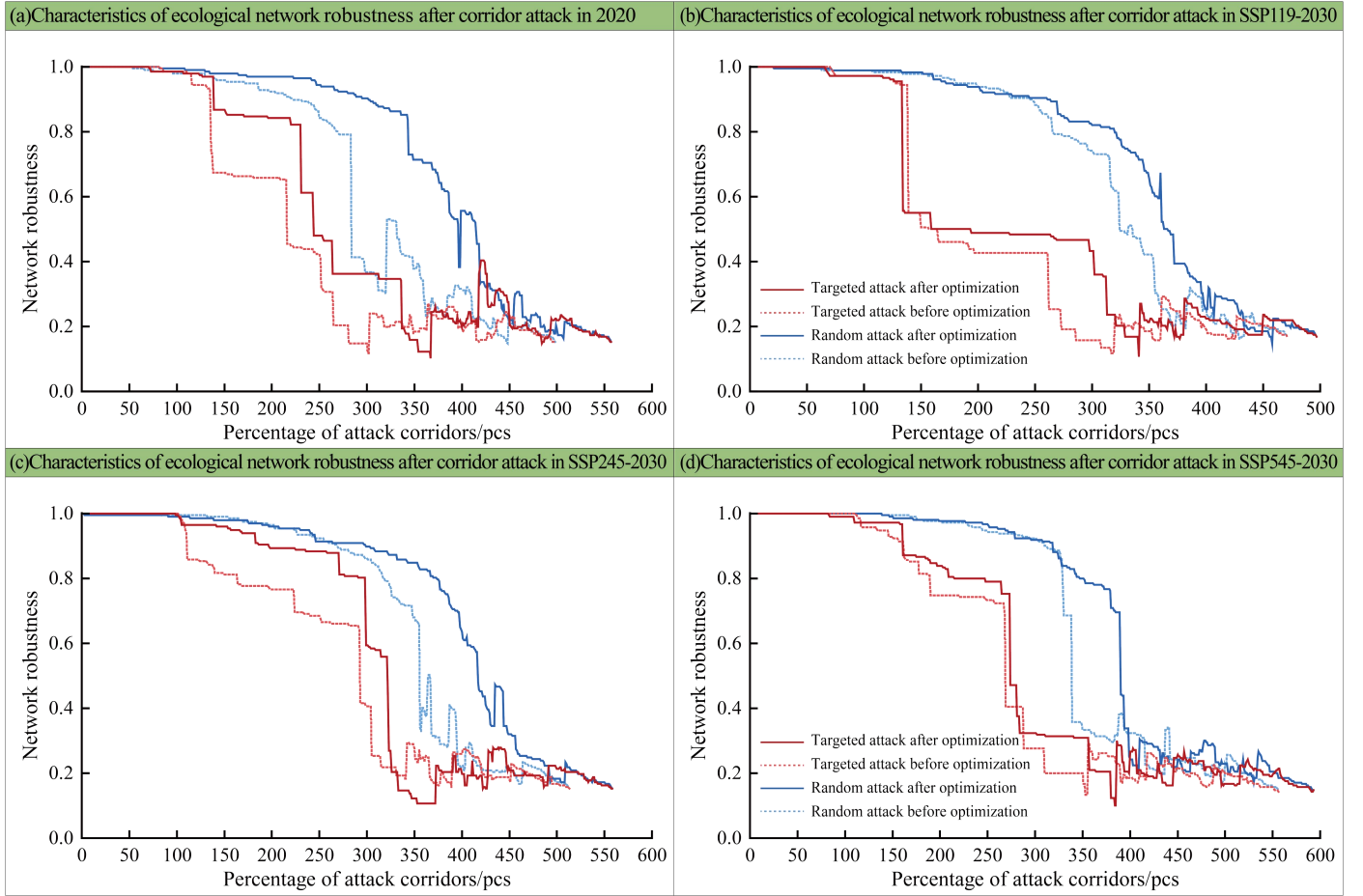
Supplementary Fig. S4 Characteristics of ecological network stability changes after random attacks and targeted attacks on corridor in the SRB.
