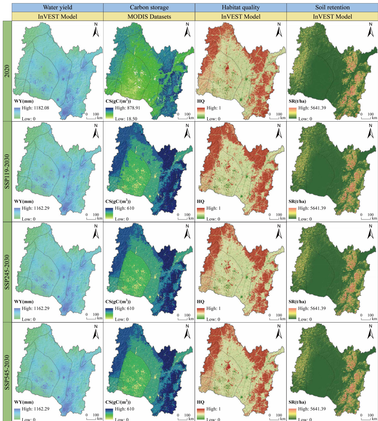
Supplementary Fig. S3 Spatial distribution of different ecosystem services in the SRB.
