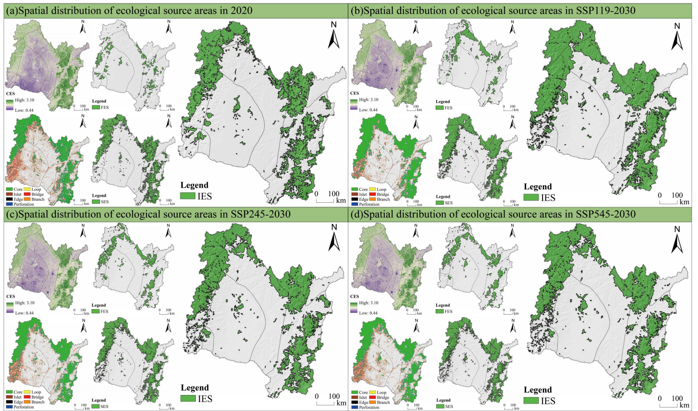
Supplementary Fig. S2 Spatial distribution of ecological source areas in the SRB. Panels (a)–(d) represent the years 2020, SSP119-2030, SSP245-2030, and SSP545-2030, respectively. FESs are derived from CESs, SESs are constructed by MSPA, and IESs are constructed by integrating the FES and the SES.
