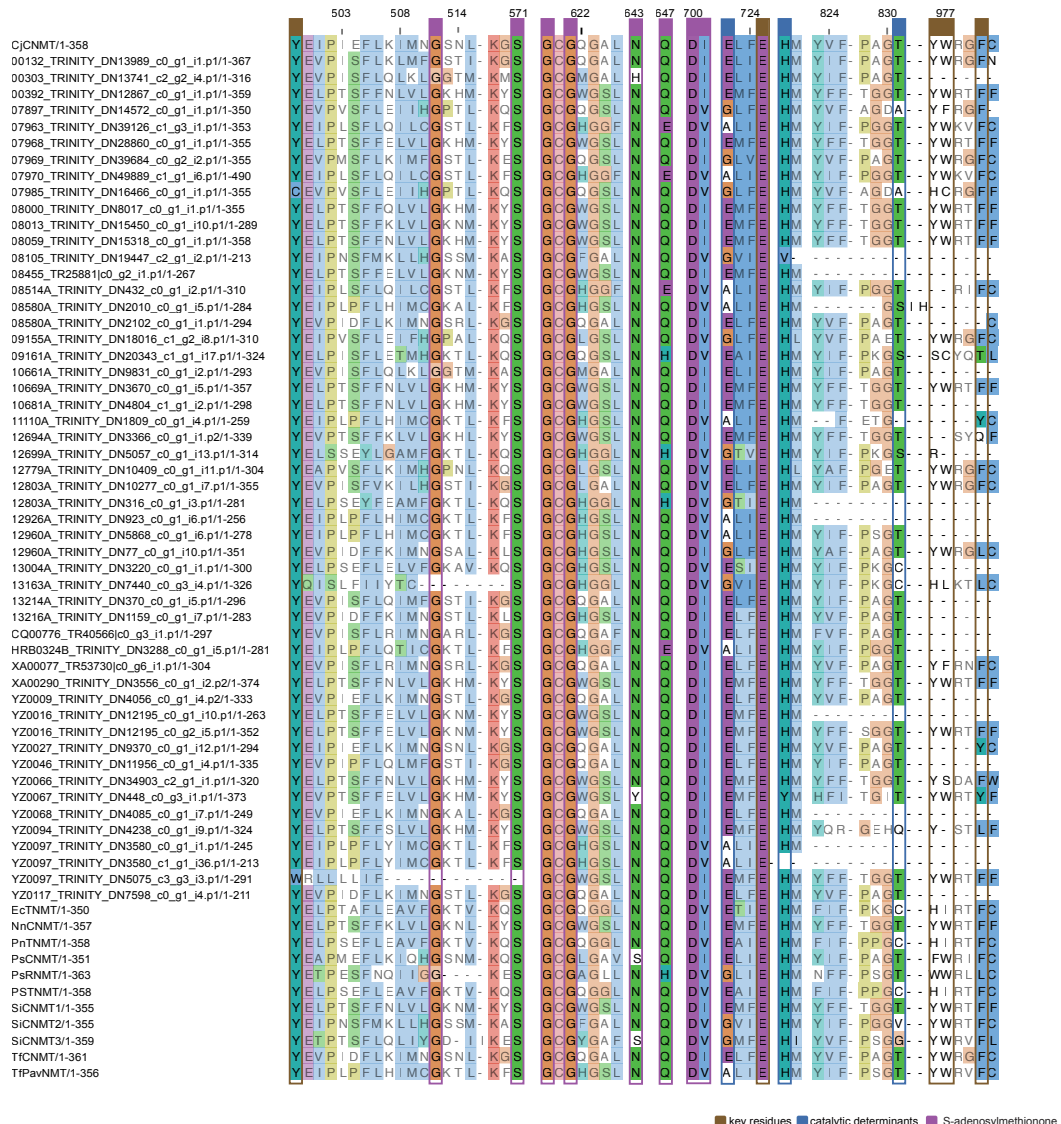
Supplementary Figure 6. Alignment of key amino acid sites in major CNMT gene family sequences. CjCNMT was used as the model, with sequences from eleven other species serving as references. The alignment includes positively selected sequences, where key residues are marked in brown, catalytic determinants in blue, and S-adenosylmethionone in purple.
