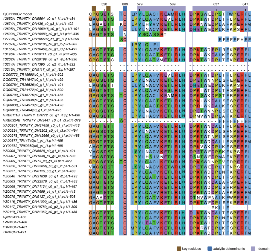
Supplementary Figure 4. Alignment of key amino acid sites in major CYP80B/NMCH genes sequences. CjCYP80G2 was used as the model, with sequences from four other species serving as references. The alignment includes positively selected sequences, where key residues are marked in brown, catalytic determinants in blue, and domains in purple.
