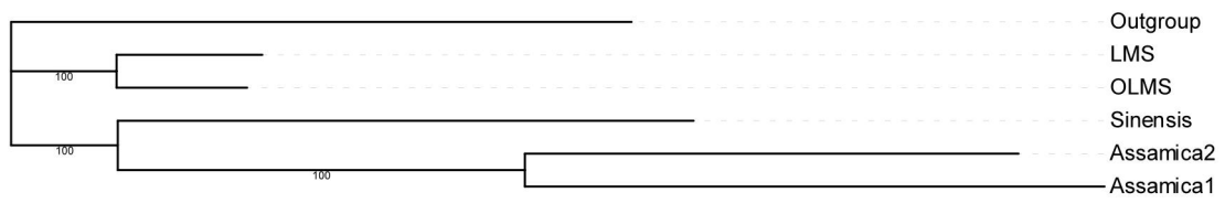
Supplementary Figure 3. Group rootless trees constructed by OLMS, LMS, global Assamica and global Sinensis. KM6 ( C. cuspidata ) was selected as the outgroup.
